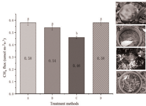
△CH 4 fluxes from mangrove soils with four different treatments.
